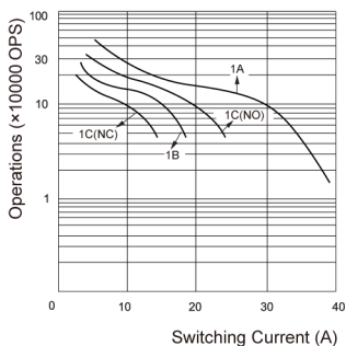
ENDURANCE CURVE
